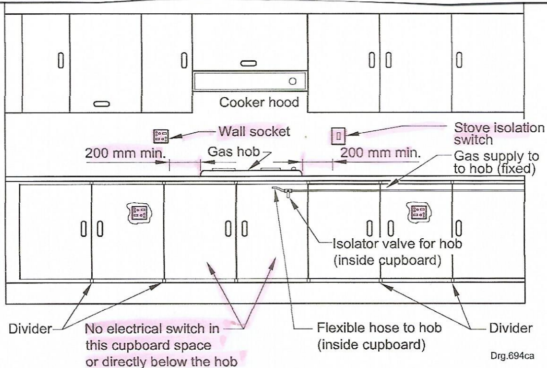
Figure 3 — Typical installation by means of a flexible hose and solid pipe
